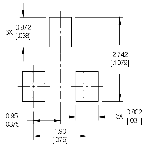
RECOMMENDED FOOTPRINT
